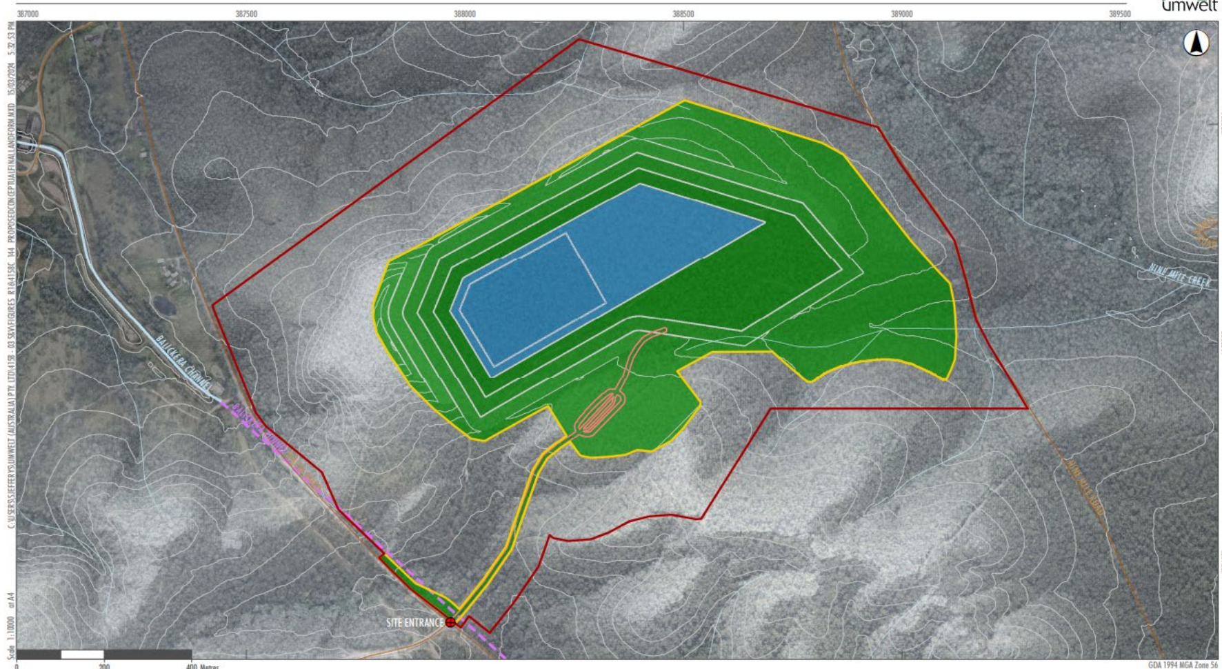
FIGURE 6.4 Proposed Conceptual Final Landform
