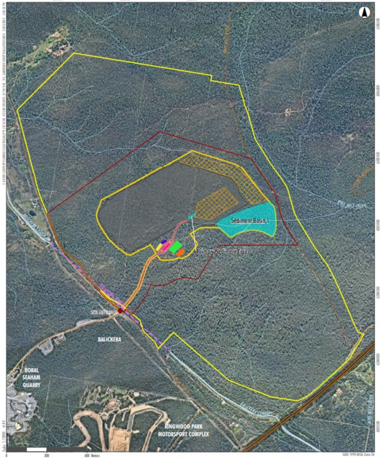
FIGURE 3.1 Amended Conceptual Quarry Layout
