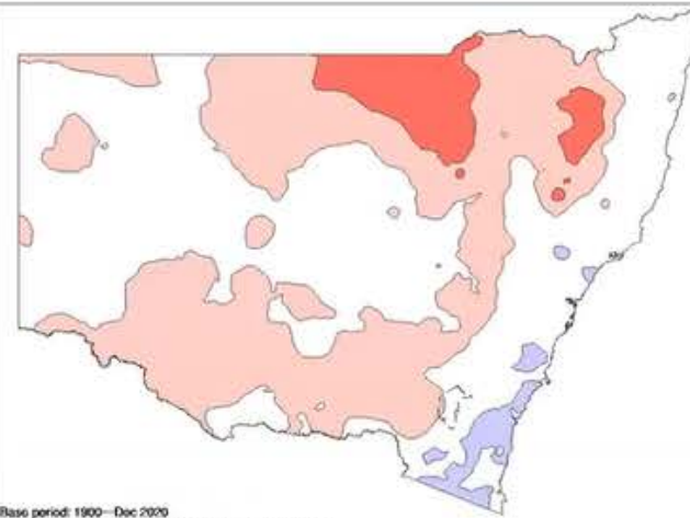
New South Wales rainfall deciles 1 January 2013 to 31 December 2014
