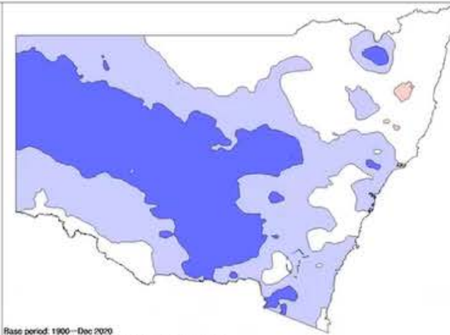
New South Wales rainfall deciles 1 January 2015 to 31 December 2016
