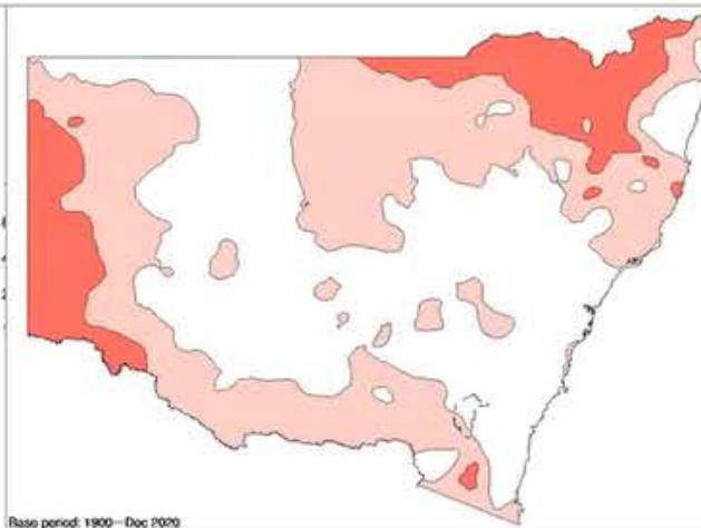
New South Wales rainfall deciles 1 January 2019 to 31 December 2020
