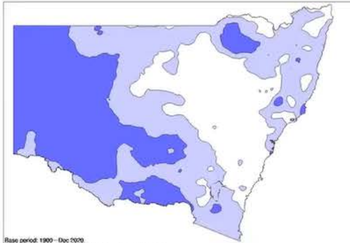
New South Wales rainfall deciles 1 January 2011 to 31 December 2012
