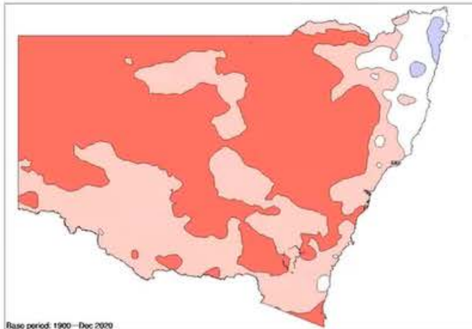
New South Wales rainfall deciles 1 January 2017 to 31 December 2018
