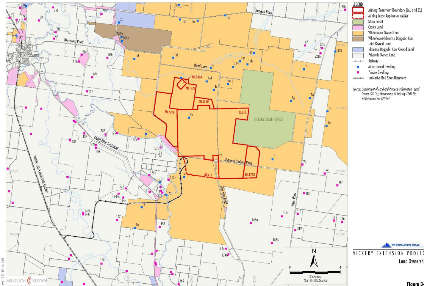
Figure 4: Receiver locations
