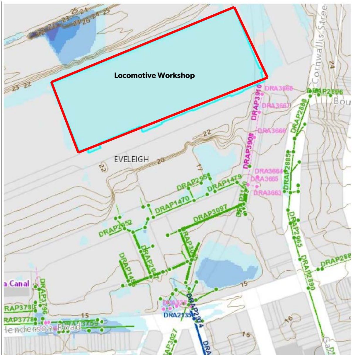
Figure 3: Extract of Council’s water assets database, with Mirvac controlled pipes in green and Sydney Water in blue.
