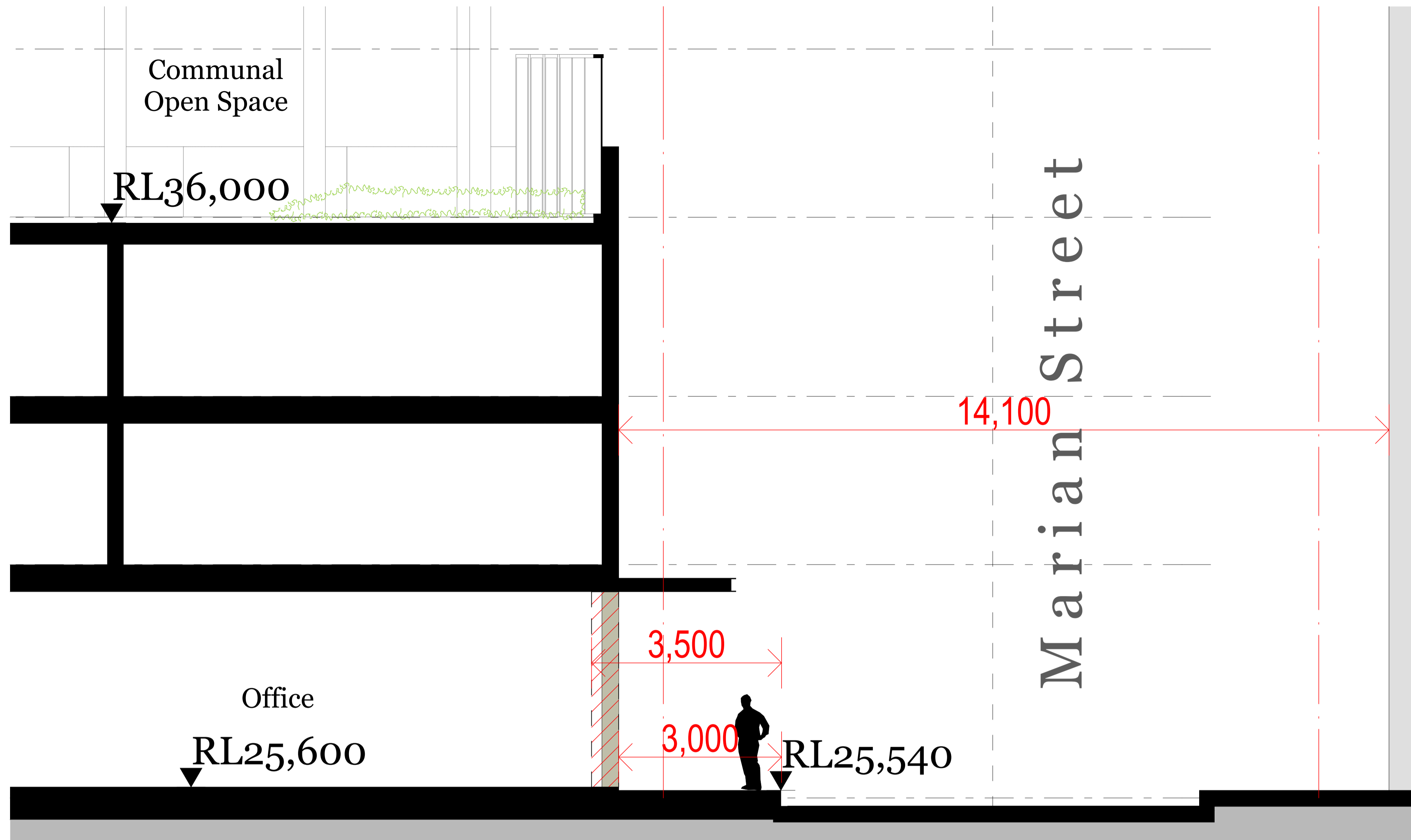
Marian Street Cross Section
