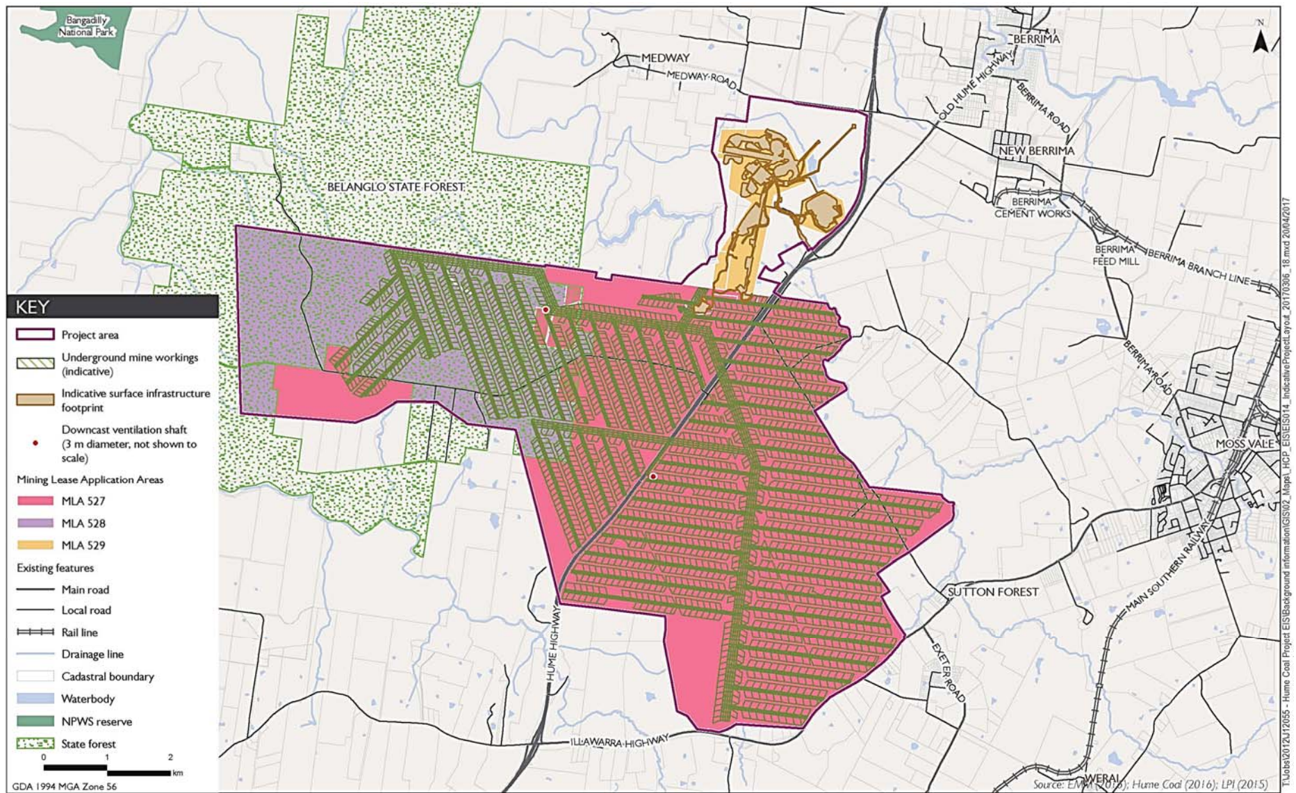
Figure 3 | Indicative layout of the Hume Coal Project
