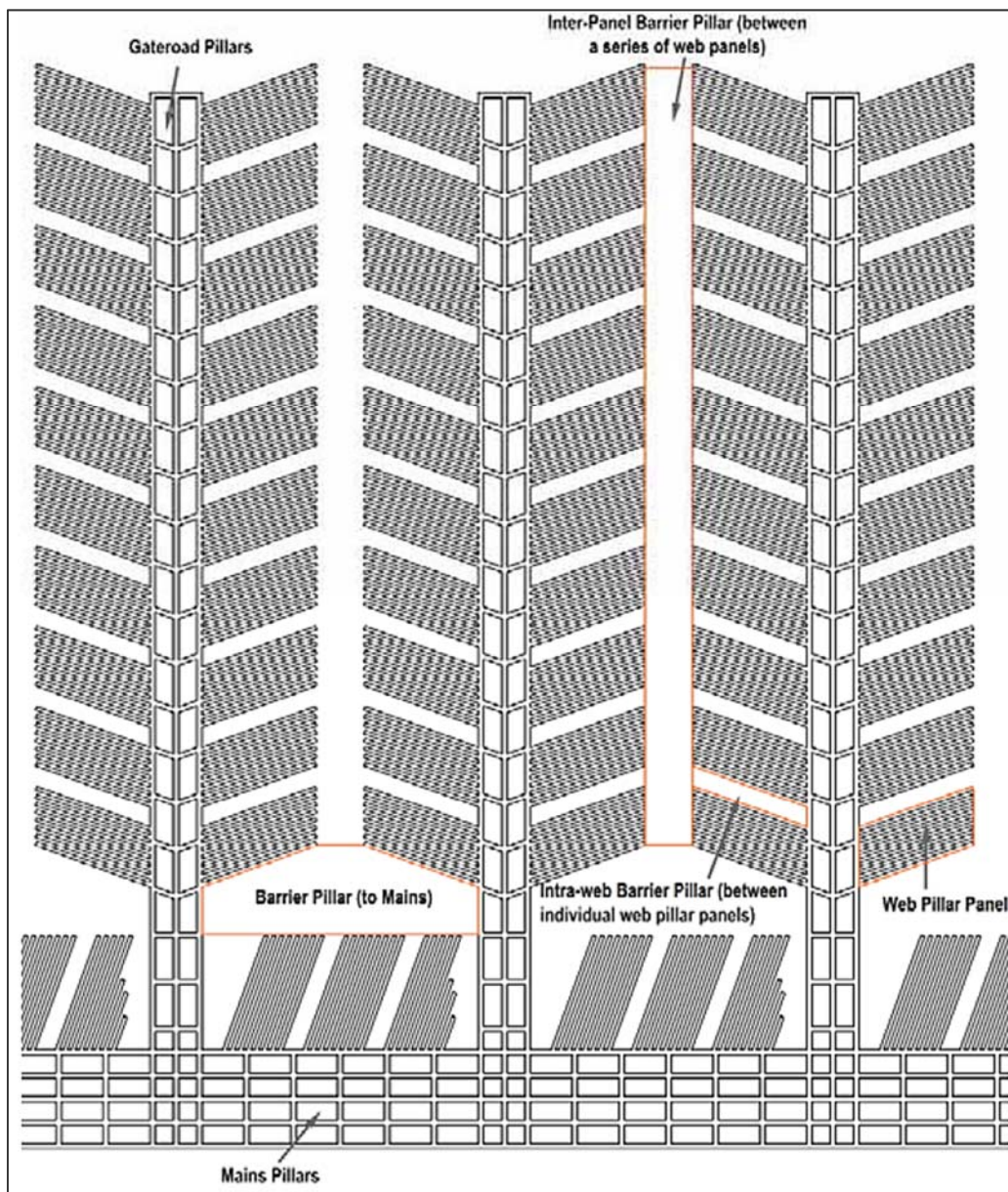
Figure 12 | Pillar types in the 'pine feather' mining method
