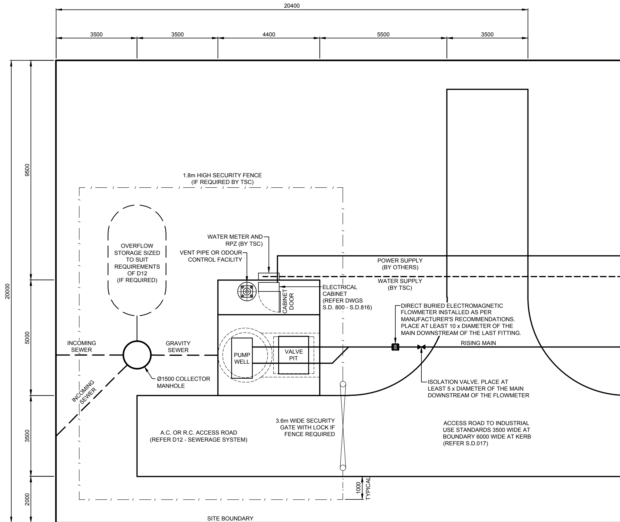
TYPICAL SITE LAYOUT SCALE 1:50 (A1) 1:100 (A3)
