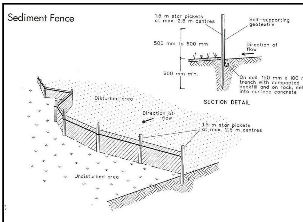
Figure 8 – Generic installation detail of geotextile filter fence
