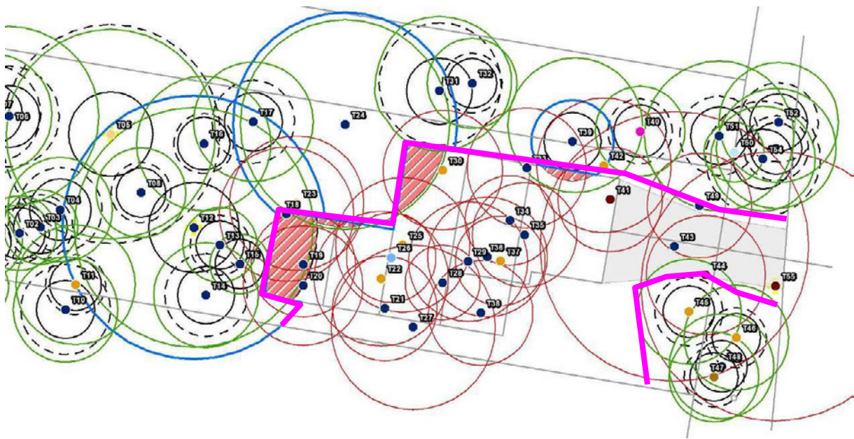
Figure 5 - Typical example of location of TPZ fencing (shown as pink line)
