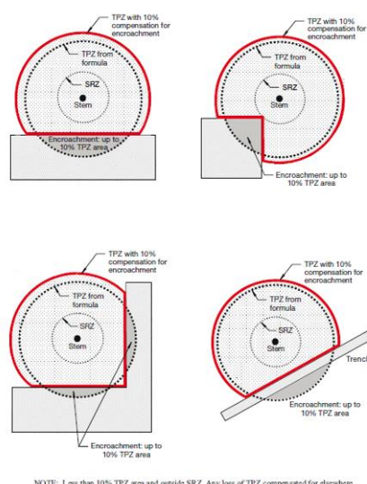
Figure 3 - Minor encroachment on TPZ and 10% compensation for encroachment (Source AS 4970-2009)
