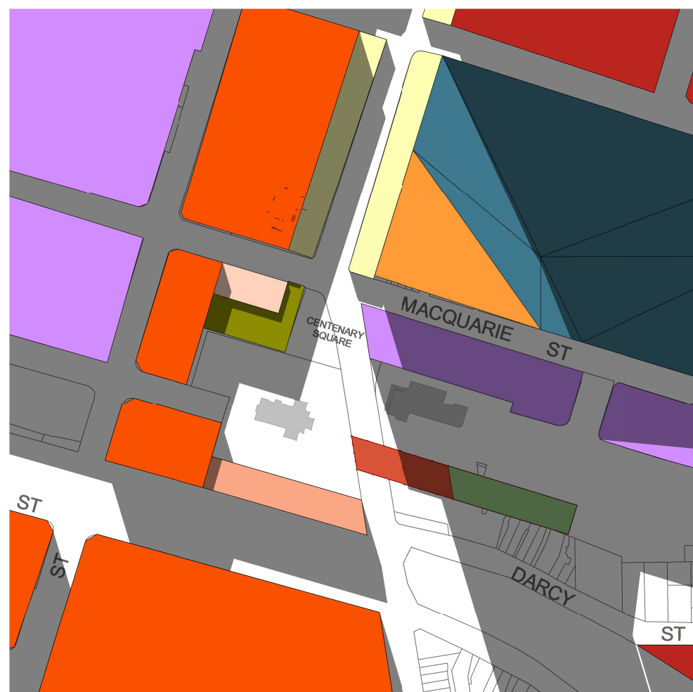
5 Shadow Analysis - 13:00pm
