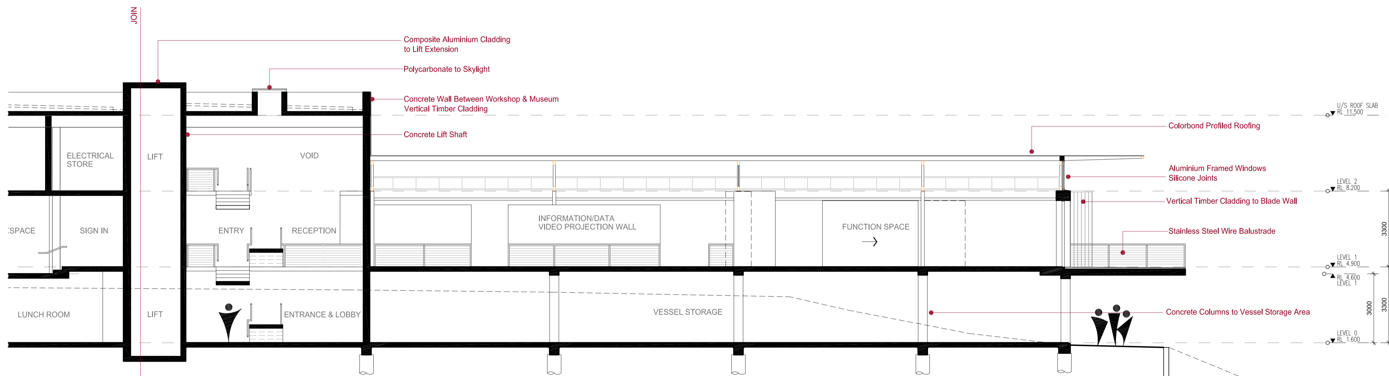
PART SECTION EE
